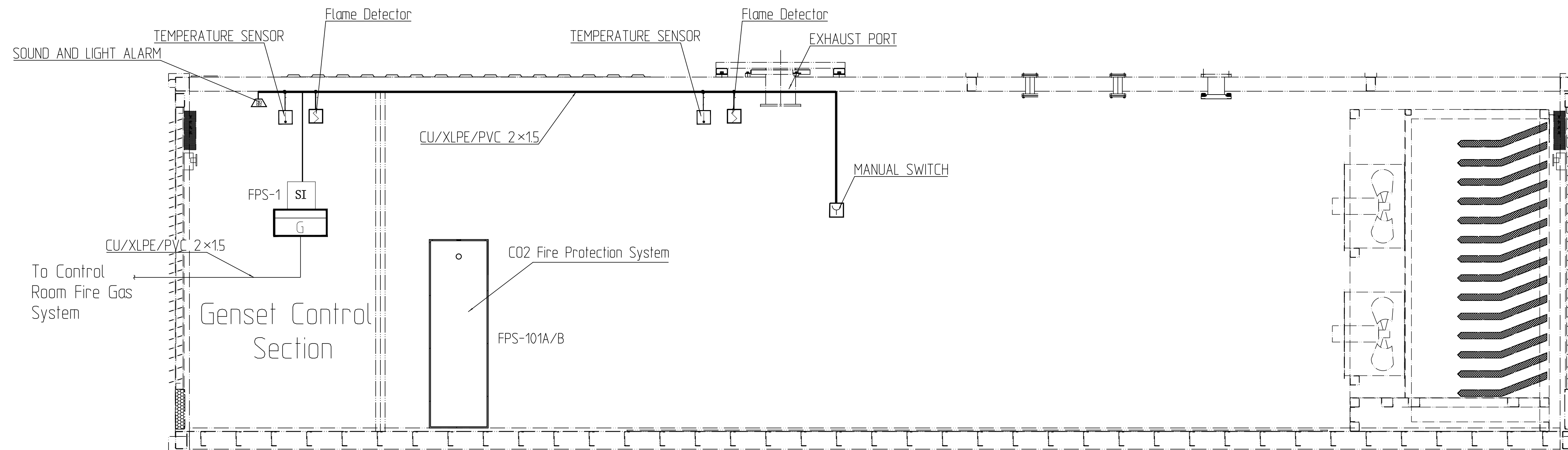
CON-1 PLAN VIEW
